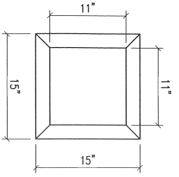
CONCRETE BLOCK FRONT VIEW
