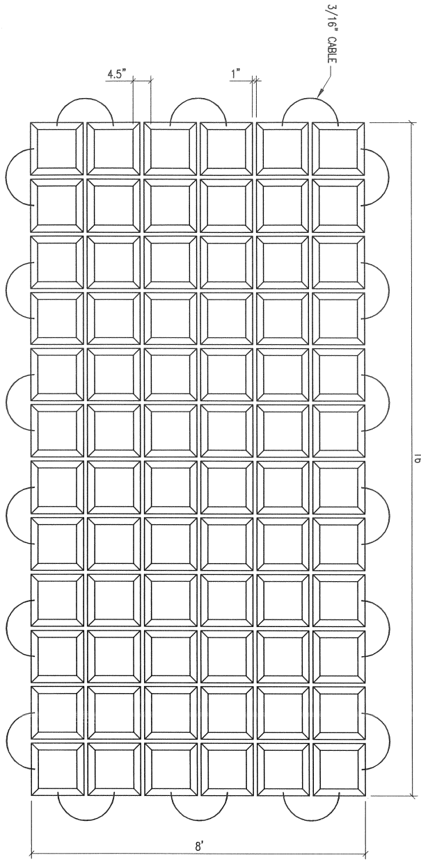
CONCRETE BLOCK REVETMENT
